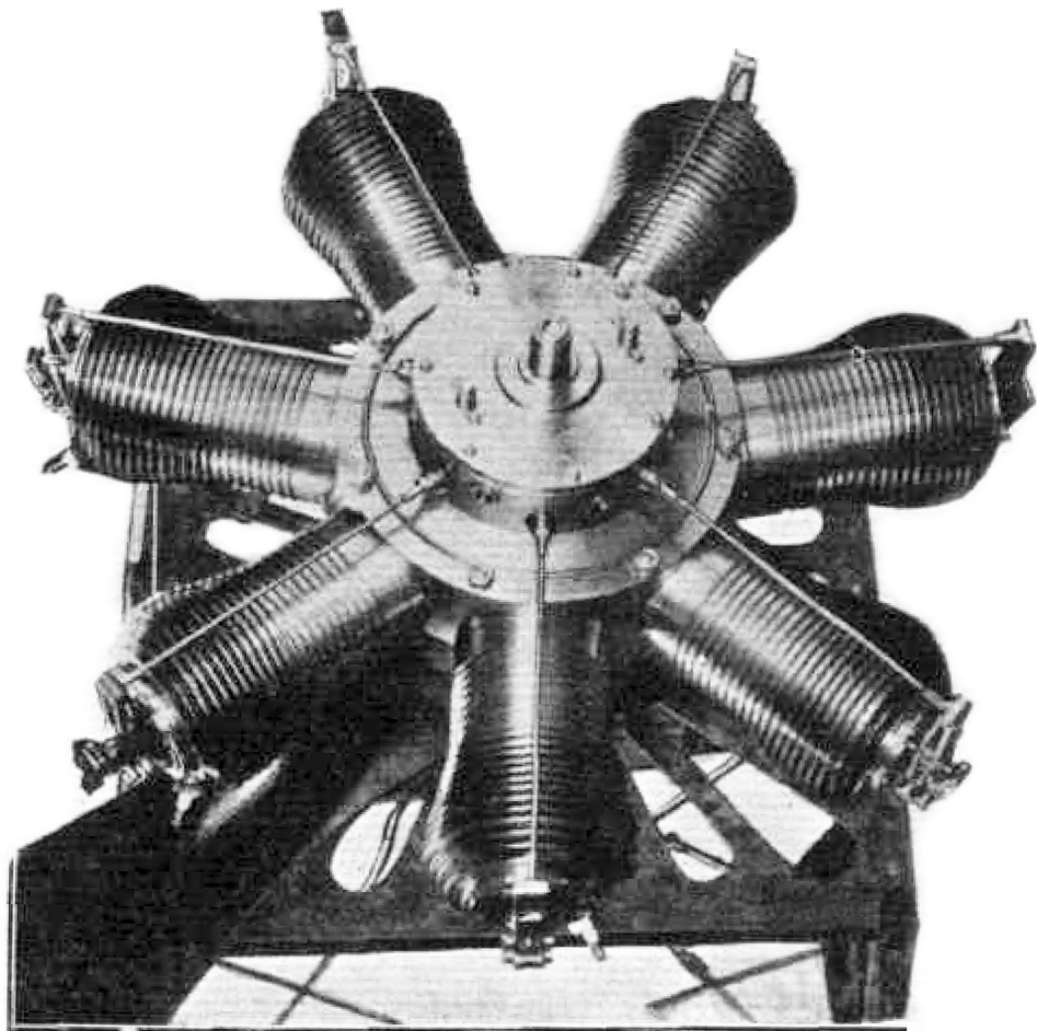
GNOME ROTARY ENGINE. —The cylinders rotate bodily with their crank-chamber about a fixed crank-shaft. All the pistons are coupled to the same crank.
